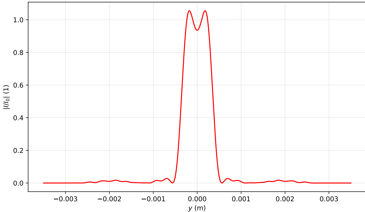
Intensity profile I(x = 0, y, z = 3.105)/I_0 , P_{in}=2.0P_{cr} , artificial time
